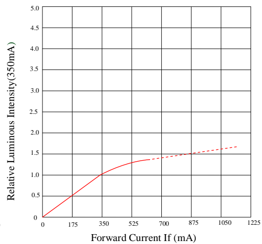
Fig.4 Iv Vs If (Ta=25°C)
